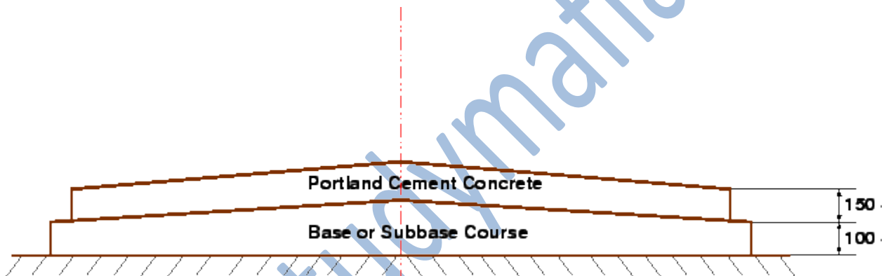
Figure 3: Typical Cross section of Rigid pavement
