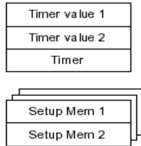
Figure 3: Timer and associated setup memories: The timer allows multiple timer periods. The different setup memories allow multiple data path configurations per event. Energy-driven operation is facilitated by multiple banks of setup memory facilitated
