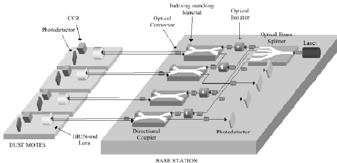
Figure 4: Fiber-optic Communication Setup
