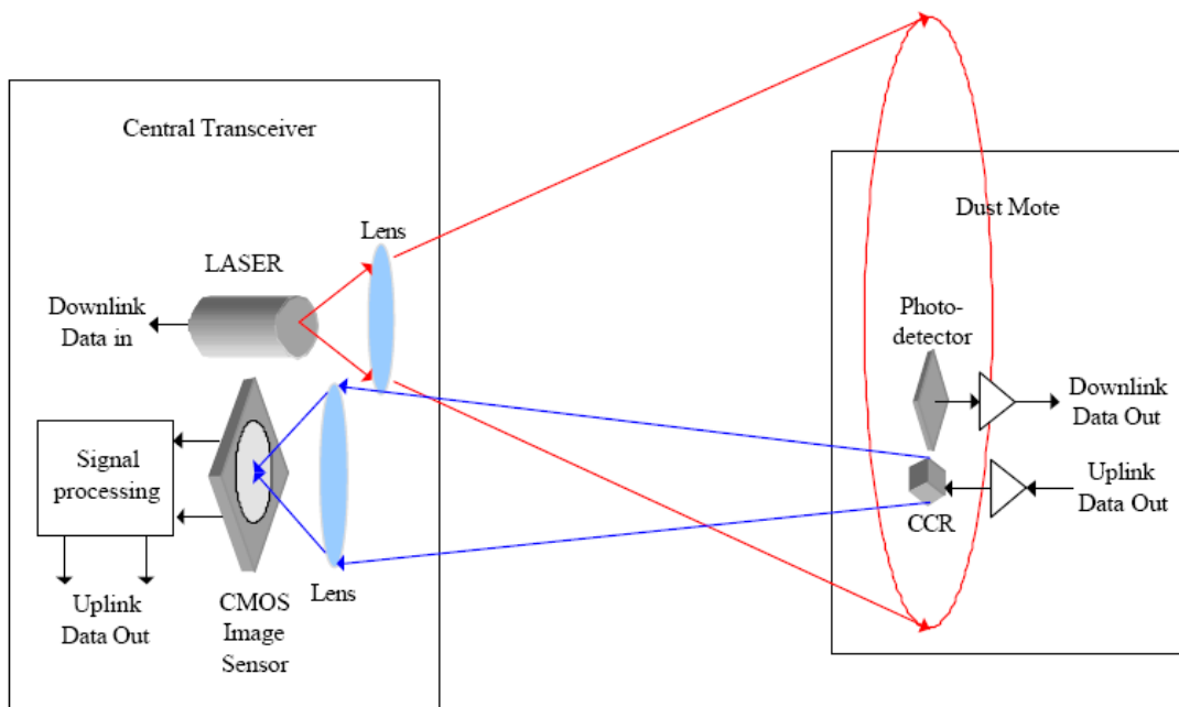
Figure 4 Free Space Optical Network
