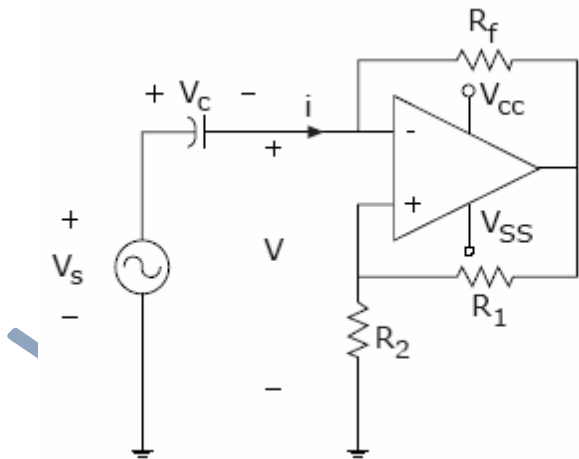
Cellonics Circuit
